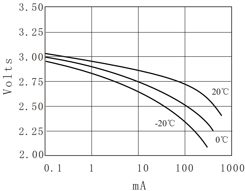
Voltage plateau versus Current and Temperature
