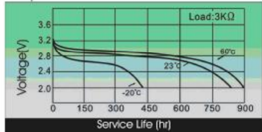
Temperature Characteristics
