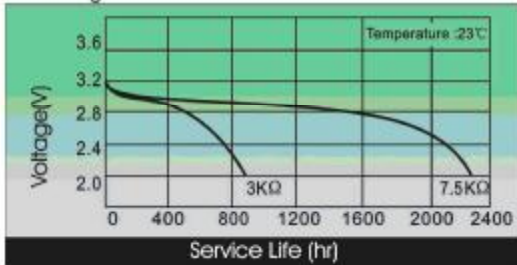
Discharge Characteristics
