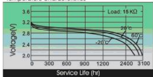
Temperature Characteristics
