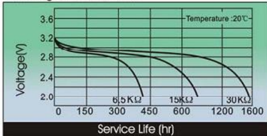
Discharge Characteristics
