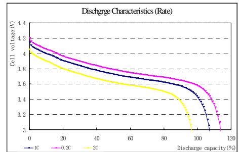
Figure 2 Discharge Characteristic
