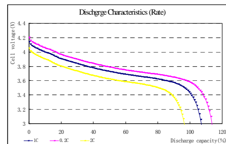
Figure 2 Discharge Characteristic
