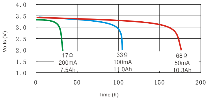
Typical discharge at 150°C
