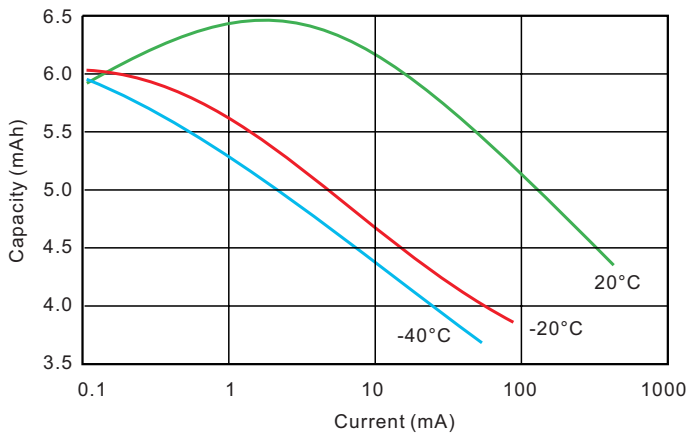
Capacity versus Current and Temperature
