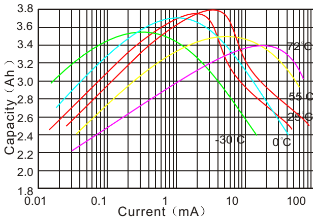
Capacity versus Current and Temperature
