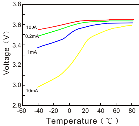
Voltage plateau versus Current and Temperature
